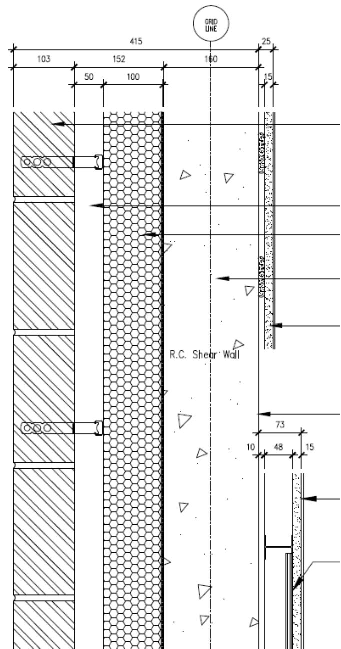
Plan Detail – Typical external wall
