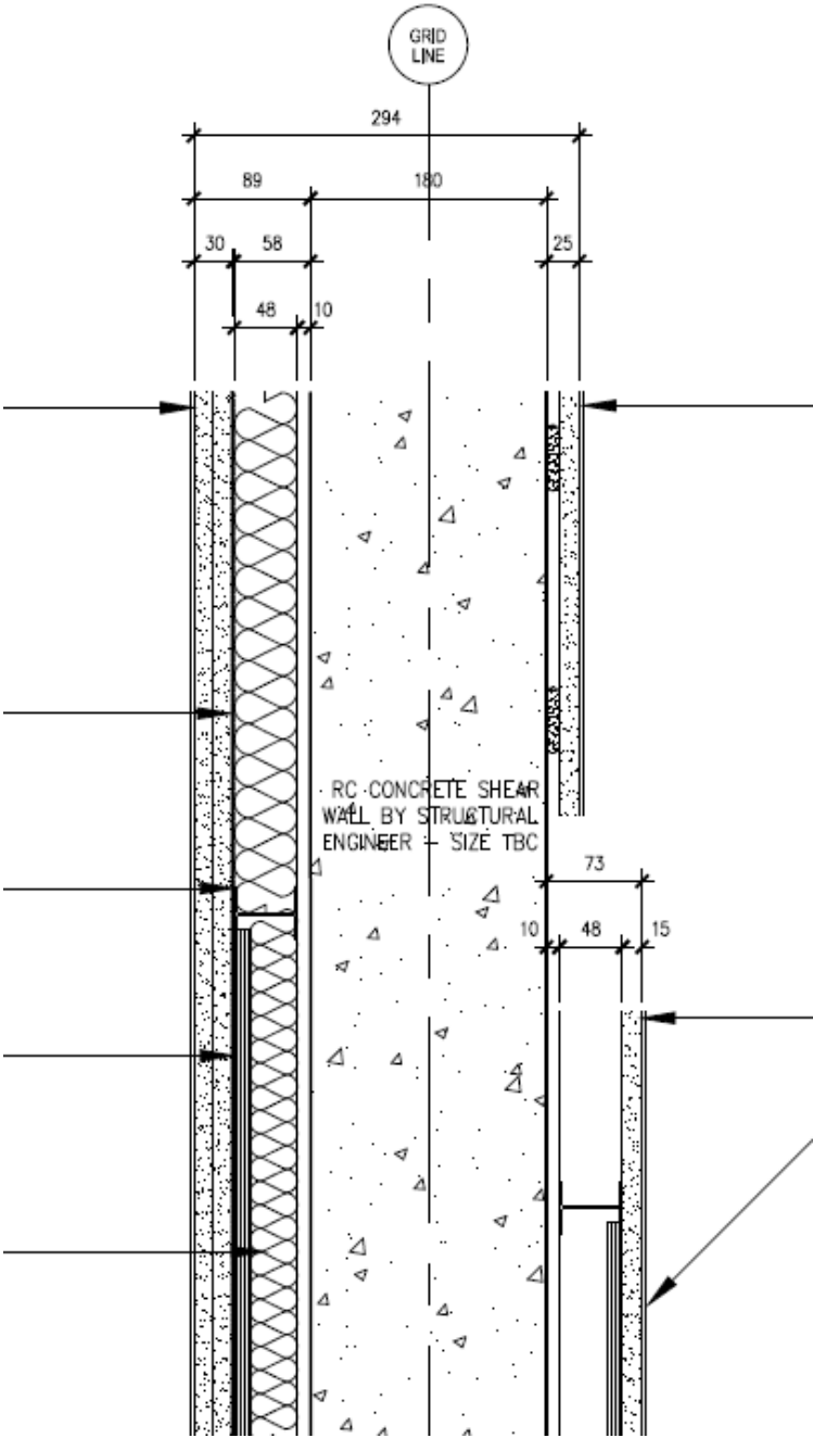
Plan Detail – Typical Party Wall (Flat to Flat)
