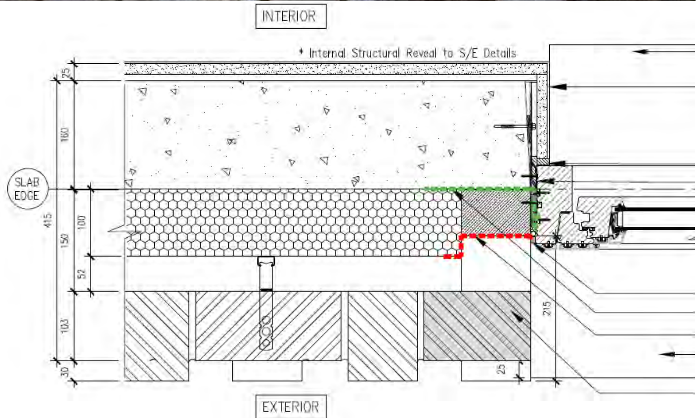
Plan Detail – Typical Window Interface – Projecting headers
