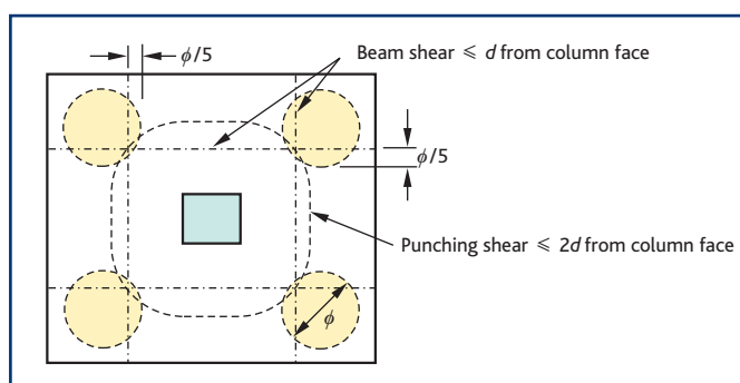
Figure 7 Shear reinforcement for pilecaps
