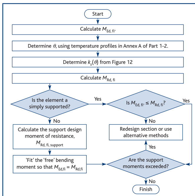
Figure 11 Flow chart for simplified calculation method for beams and slabs
