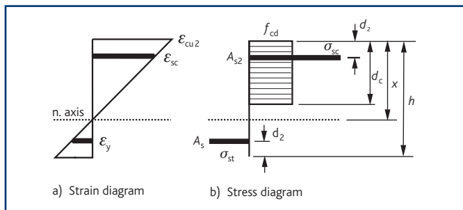
Figure 8 Stress block diagram for columns
