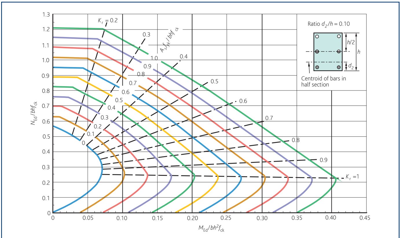
Figure 10b Column design chart for rectangular columns d_2/h = 0.10
