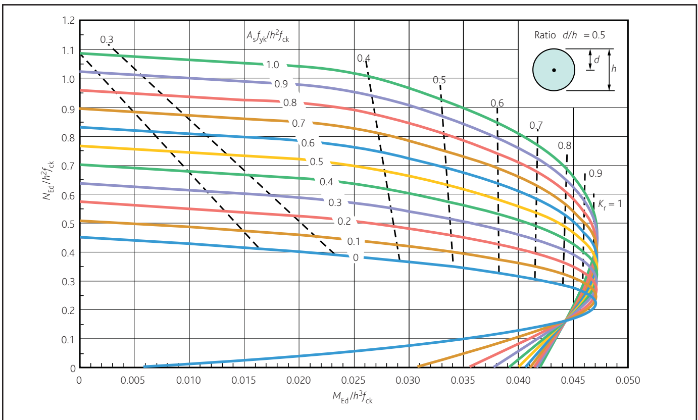
Figure 11a Circular columns ( f_{ck} < 50 \text{ MPa} , f_{yk} = 500 \text{ MPa} ) d/h = 0.5
