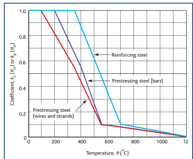
Figure 12 Reference curves for critical temperature of reinforcing and prestressing steel for use with tabular method and Annex E
