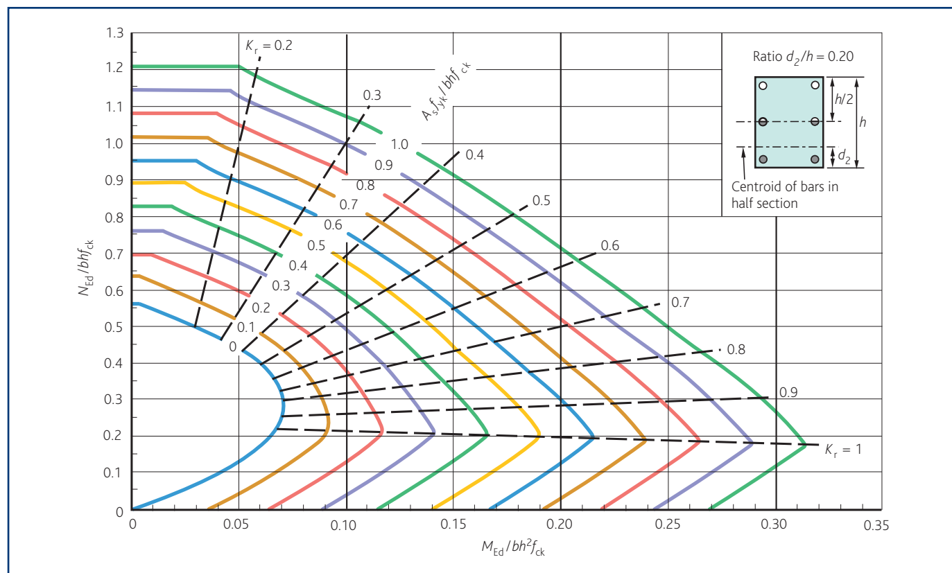
Figure 10d Column design chart for rectangular columns d_2/h = 0.20
