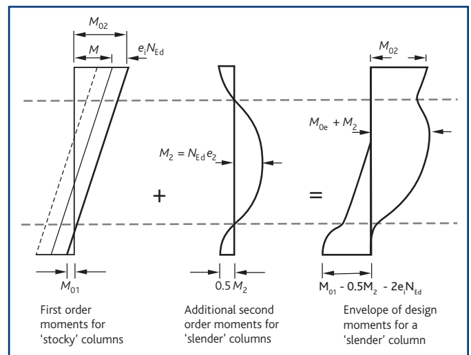
Figure 4 Design bending moments for a braced slender column
