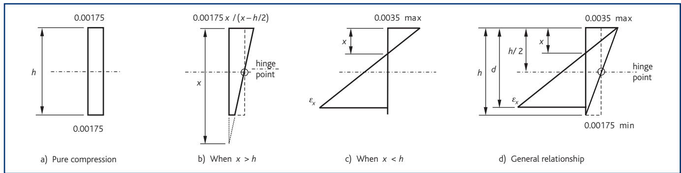
Figure 9 Strain diagrams for columns
