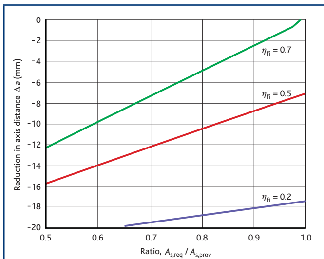
Figure 8 Reduction in axis distance, a , depending on area of steel provided
