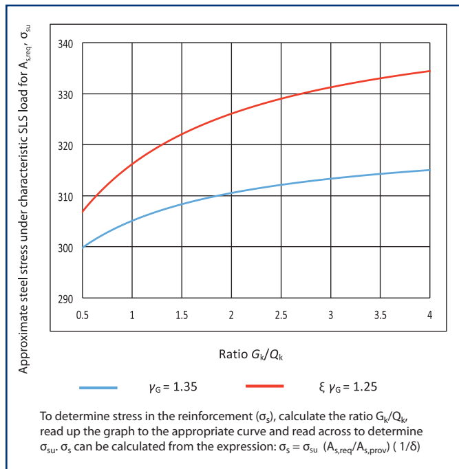
Figure 5 Determination of approximate steel stress at SLS
