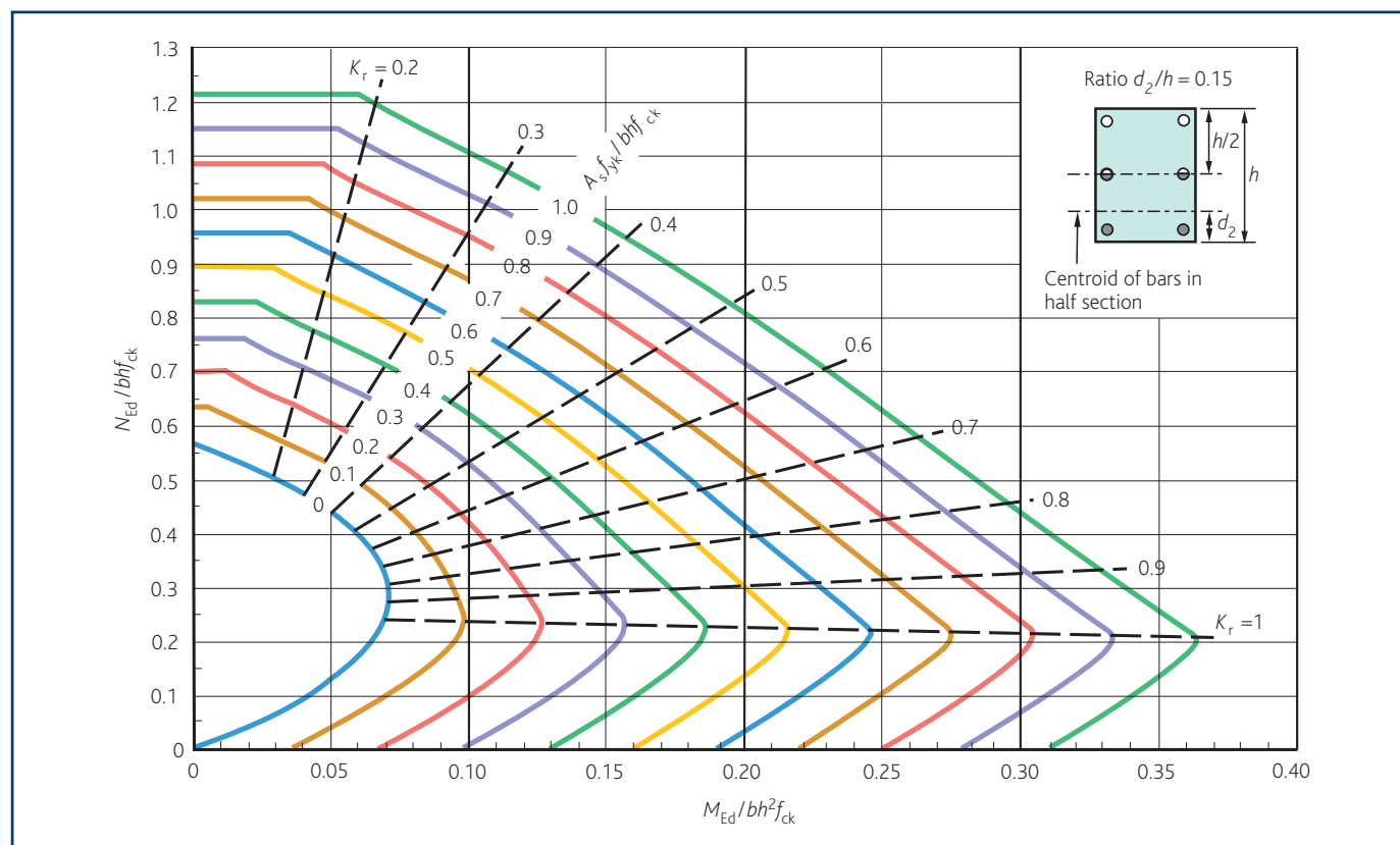
Figure 10c Column design chart for rectangular columns d_2/h = 0.15
