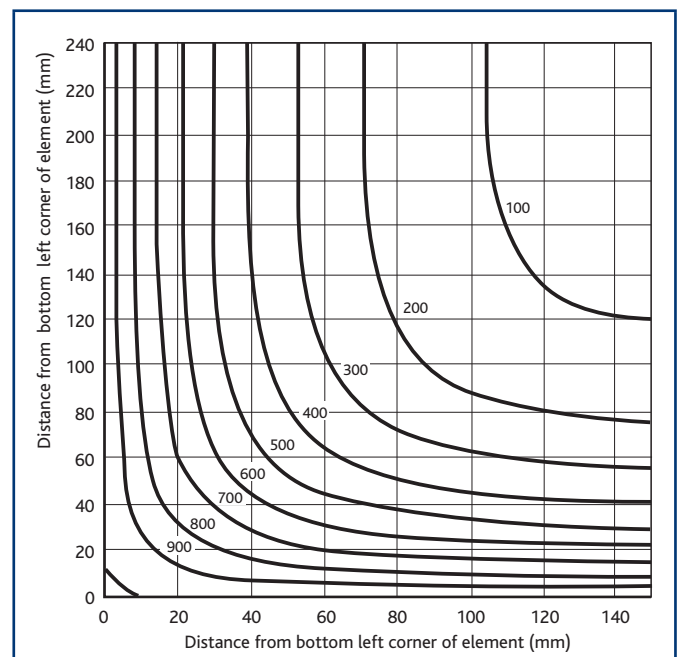
Figure 14 Example temperature profile for a 600 x 300 beam and R90
