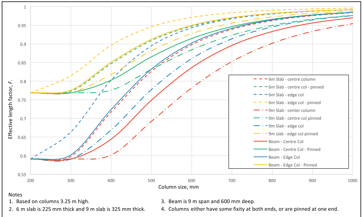
Figure 6 Effective length factor, F , for braced columns
