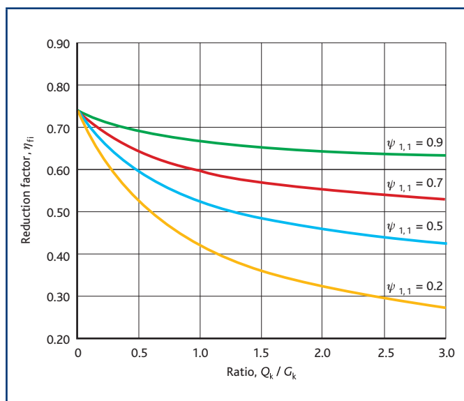
Figure 5 Determination of \eta_{fi} using Expression 2.5 of Part 1-2
