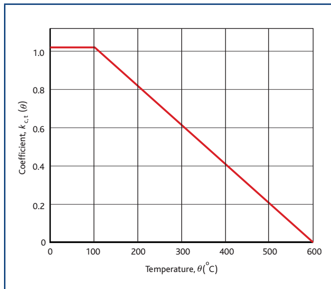
Figure 17 Coefficient k_{c,t}(\theta) allowing for decrease of tensile strength ( f_{ck,t} ) of concrete at elevated temperatures
