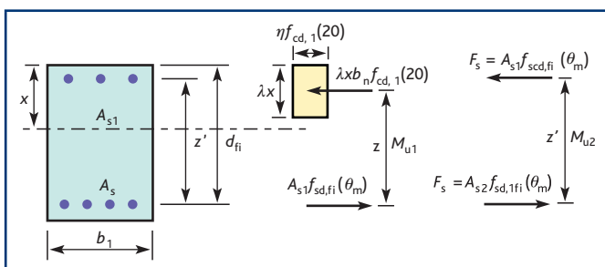
Figure 15 Stress distribution at ultimate limit state for a rectangular concrete cross-section with compression reinforcement.
