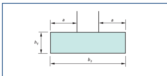
Figure 8 Dimensions for plain foundations
