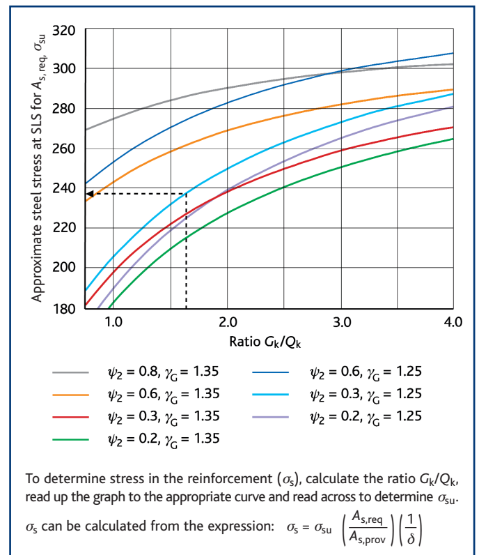
Figure 8 Determination of steel stress for crack width control
