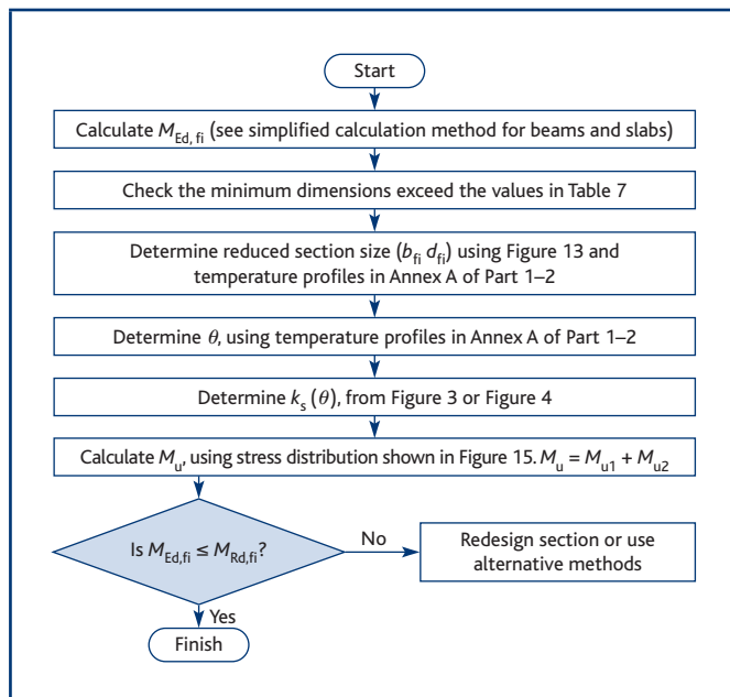
Figure 16 Flow chart for 500°C isotherm method
