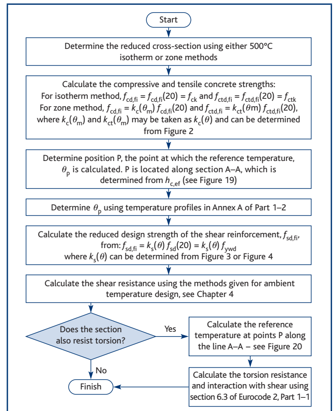
Figure 18 Design flow chart for shear and torsion design
