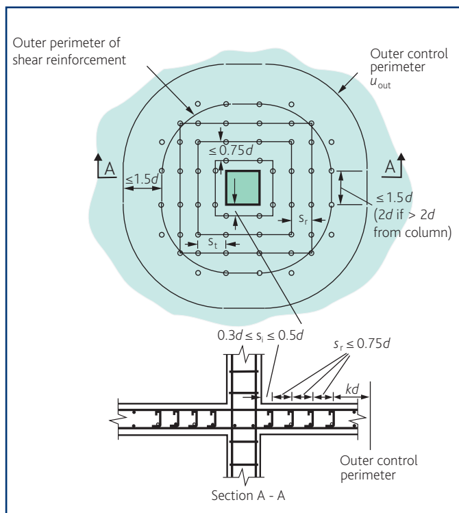
Figure 9 Punching shear layout
