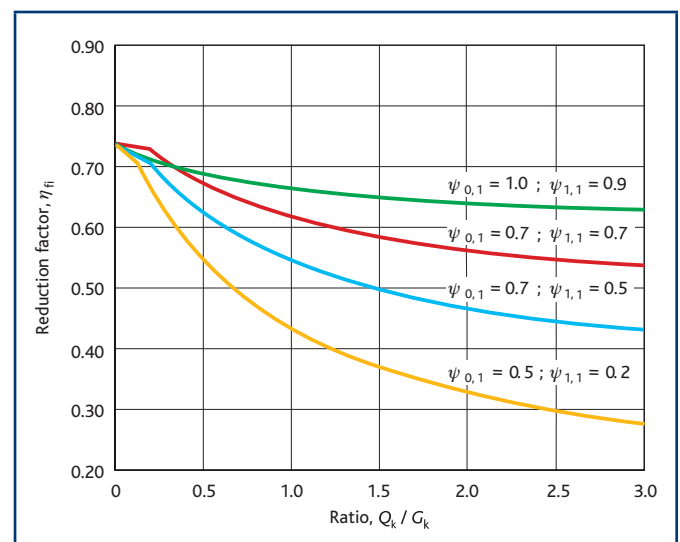
Figure 6 Determination of \eta_{fi} using Expressions (2.5a and b) of Part 1-2
