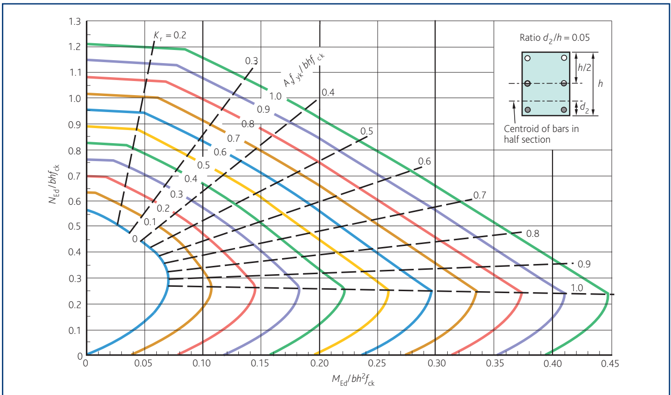
Figure 10a Column design chart for rectangular columns d_2/h = 0.05
