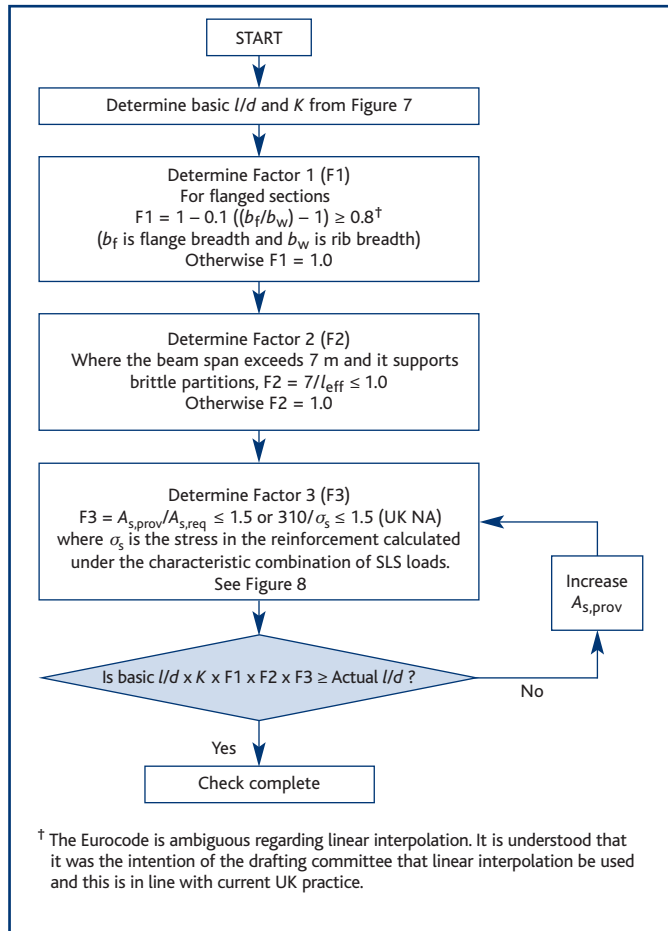
Figure 6 Procedure for assessing deflection
