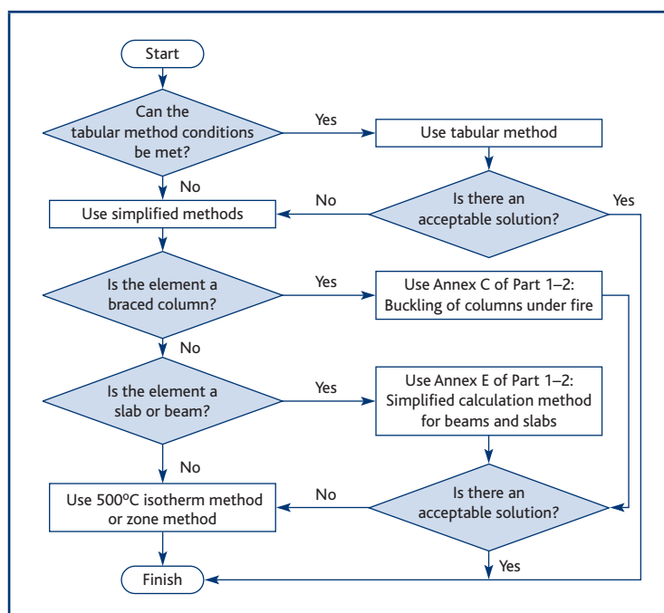
Figure 1 Flow chart showing which fire resistance design method to adopt
