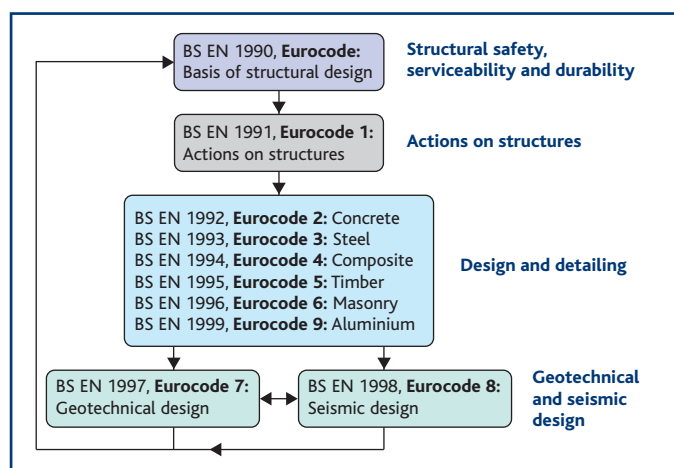
Figure 1 The Eurocodes
