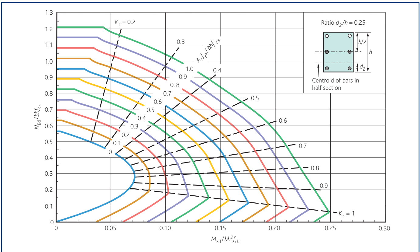
Figure 10e Column design chart for rectangular columns d_2/h = 0.25
