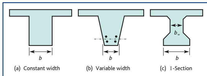
Figure 9 Definition of dimensions for different types of beam section
