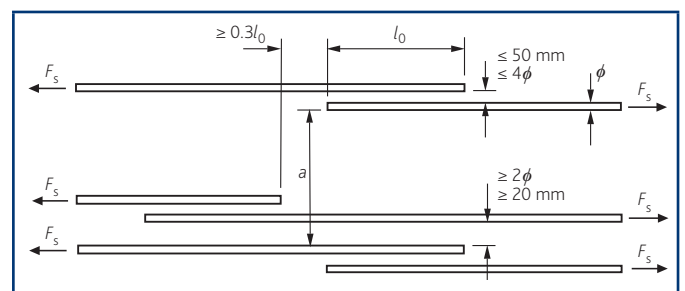
Figure 5 Arranging adjacent lapping bars
