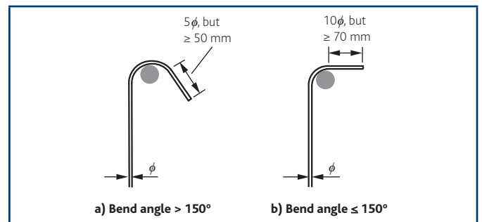
Figure 3 Anchorage of links
