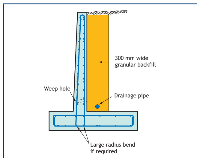
Figure 17 Typical drainage layout for a retaining wall
