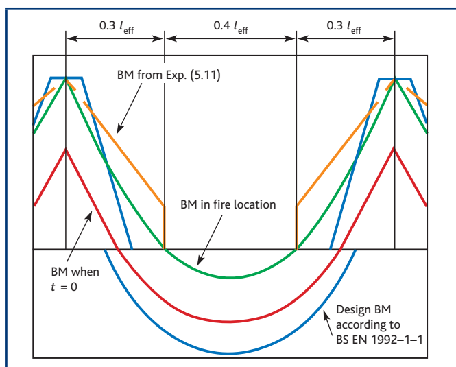
Figure 10 Envelope of resisting bending moments over supports for fire conditions
