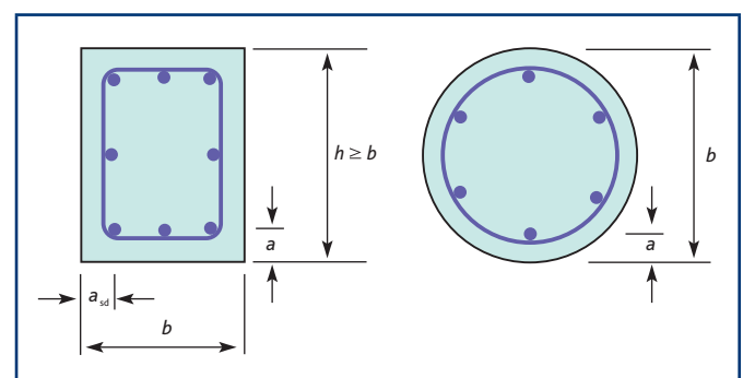
Figure 7 Section through member showing nominal axis distance, a
