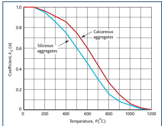
Figure 3 Coefficient k_s(\theta) allowing for decrease of characteristic strength ( f_{yk} ) of tension and compression reinforcement (class N)
