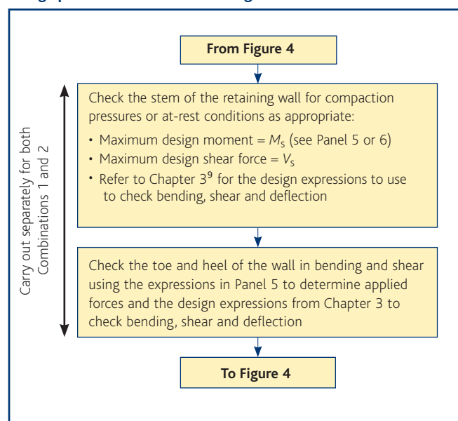
Figure 13 Design procedure for structural design
