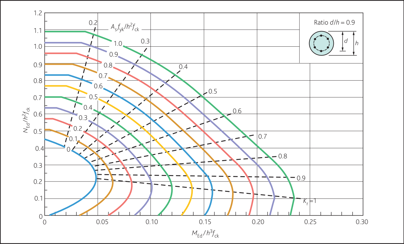
Figure 11f Circular columns ( f_{ck} \leq 50 \text{ MPa} , f_{yk} = 500 \text{ MPa} ) d/h = 0.9
