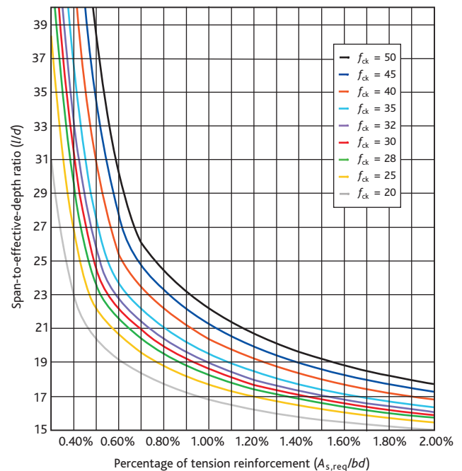
Figure 4 Basic span-to-effective-depth ratios for flat slabs
