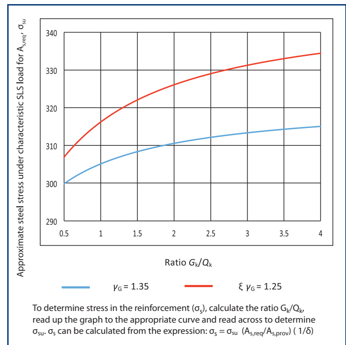
Figure 4 Determination of approximate steel stress at SLS
