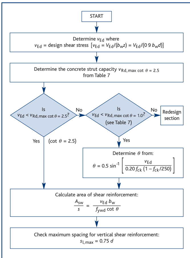
Figure 5 Procedure for determining vertical shear reinforcement
