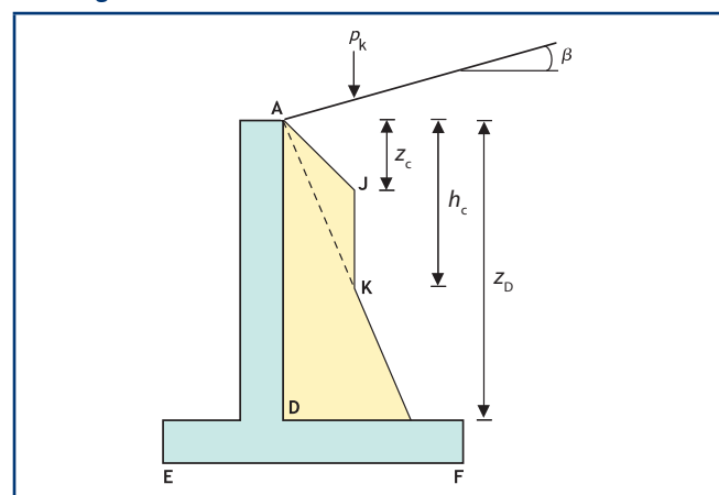
Figure 14 Compaction earth pressures for structural design of cantilever retaining walls
