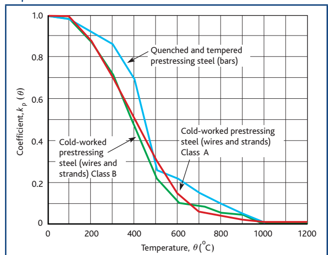
Figure 4 Coefficient k_p(\theta) allowing for decrease of characteristic strength ( \beta f_{pk} ) of prestressing steel
