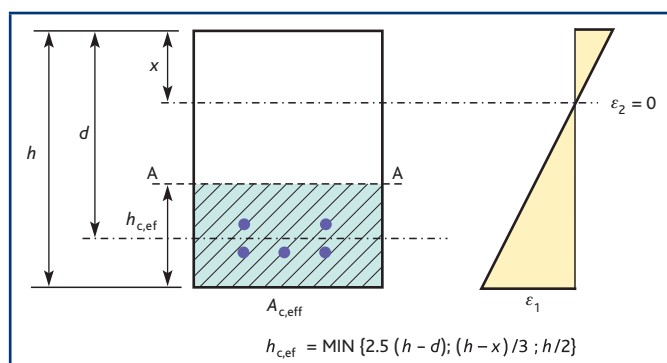
Figure 19 Determination of line A–A to enable evaluation of reference temperature \theta_p at point P
