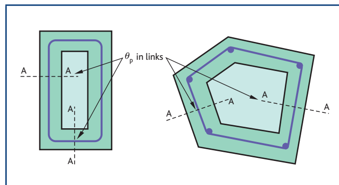
Figure 20 The reference temperature \theta_p should be evaluated along the line A–A for the calculation of torsion resistance
